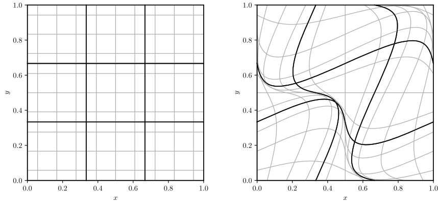
Figure 2: Meshes for N = 4 , K = 3^2 . Left: c = 0 . Right: c = 0.3 . The black lines represent element boundaries and the gray lines represent the GLL mesh.
